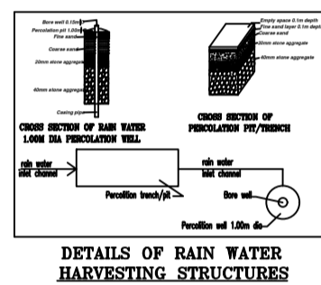
DETAILS OF RAINY WATER HARVESTING STRUCTURES
