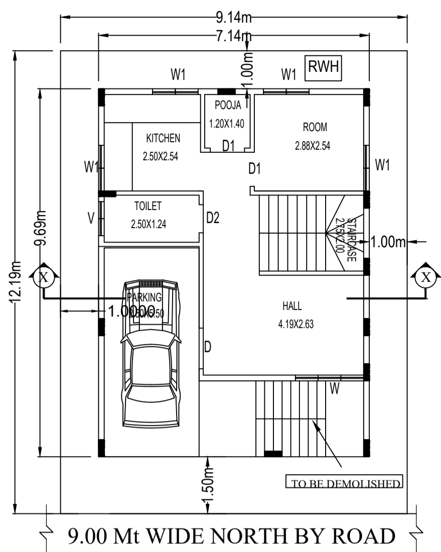
EXISTING AND ALTERED GROUND FLOOR PLAN
